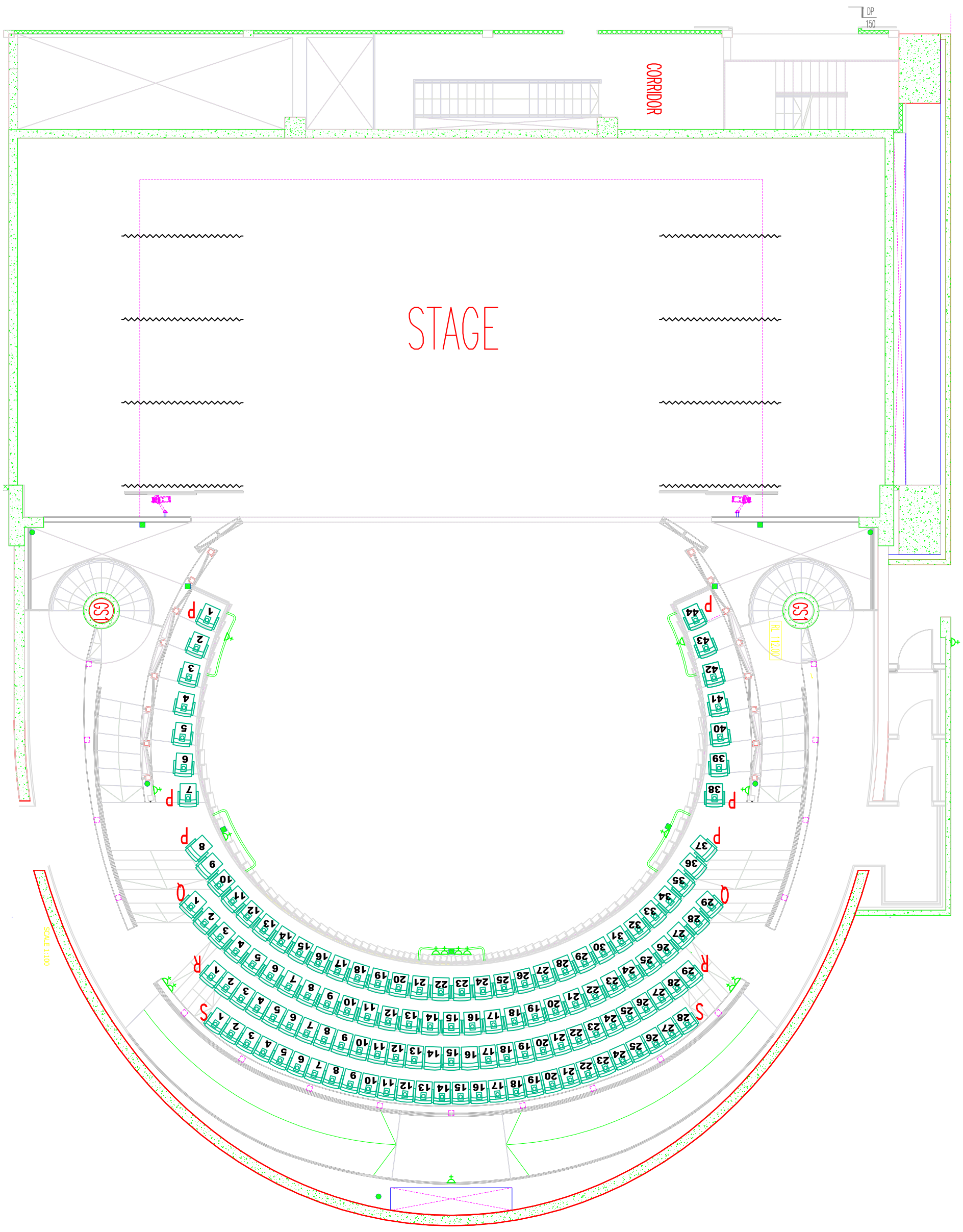
DRAMA THEATRE CIRCLE AUDIENCE SEATING - SCALE 1:200 (A3 SIZE)
